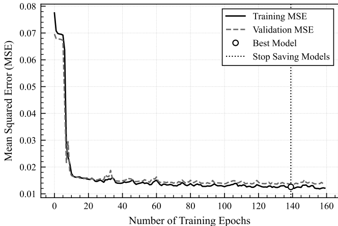
Learning Curve of TCSA-GRU Model for SolarPlant-3 (Gyeongju)
